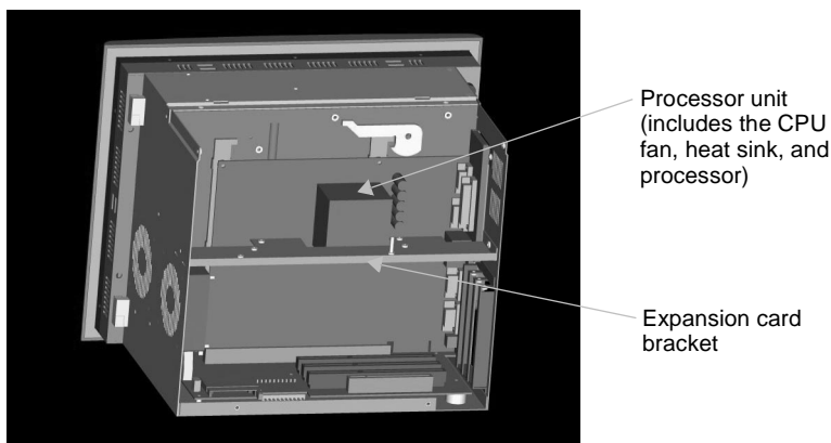
Figure 3: Processor Unit
